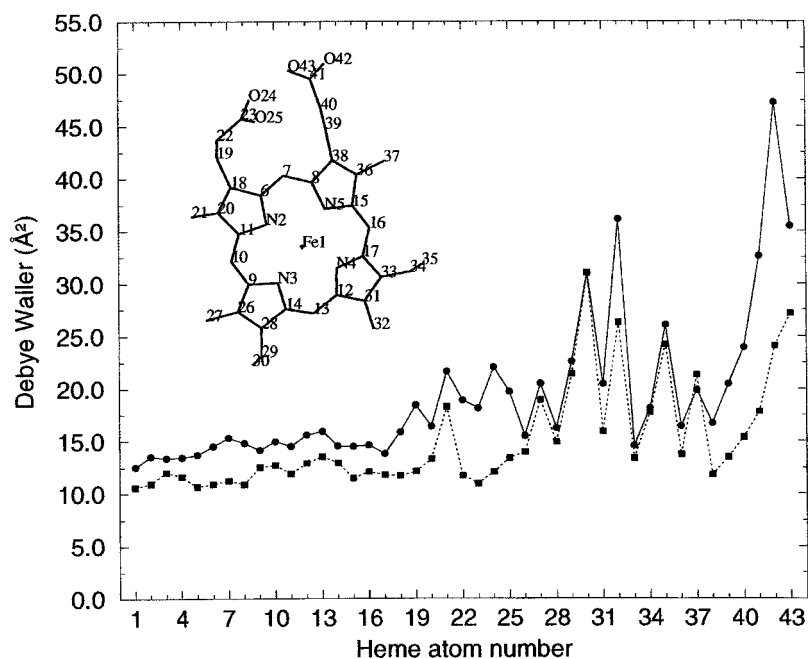
FIGURE 7 Averaged Debye-Waller factors for each heme atom of the wild-type (●), and mutant (■) deoxy S. inaequalis HbI. In the upper left of the picture is shown a scheme of the heme group where each atom is identified by a number. All the heteroatoms are explicitly labeled.
